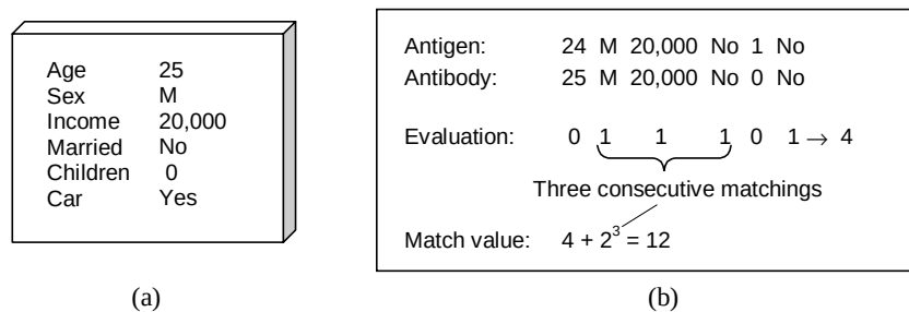
Figure 30: (a) Structure of a case (antigen or antibody). (b) The match algorithm (see Equation (12)).
