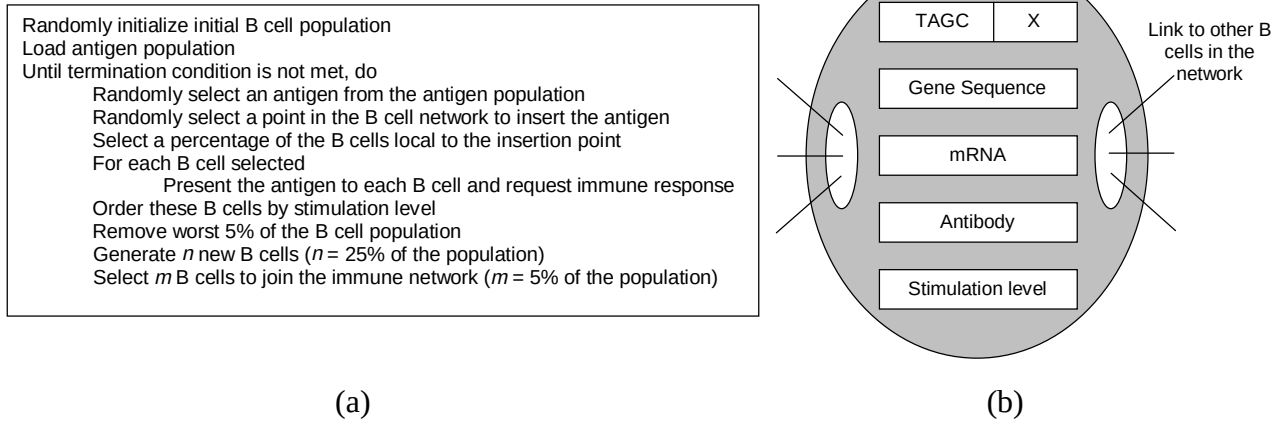
Figure 19: (a) The immune system object algorithm. (b) Structure of a B-cell object.
