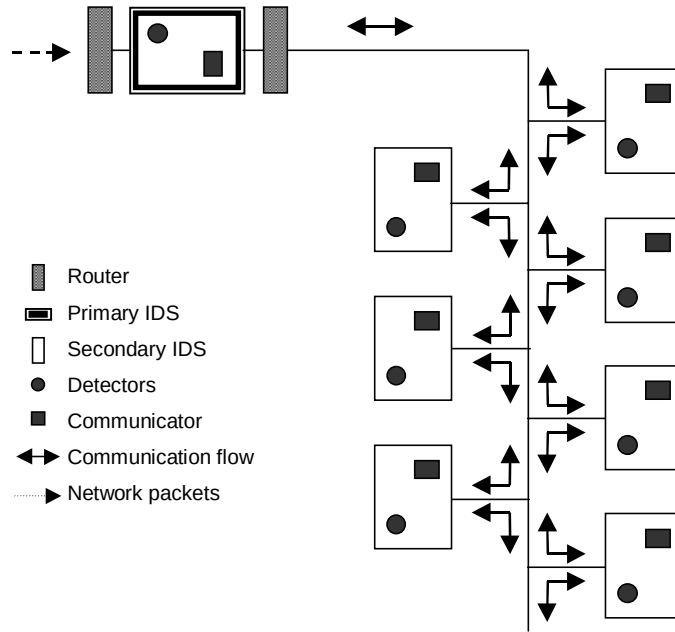
Figure 15: Physical architecture of an artificial immune system for network intrusion detection.
