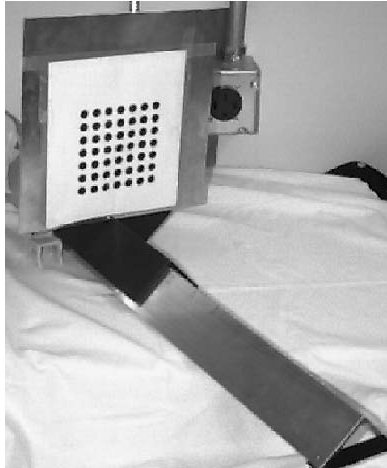
Figure 13.22: A calibration object that uses a moving 2D pattern to create many feature points in 3D space.
