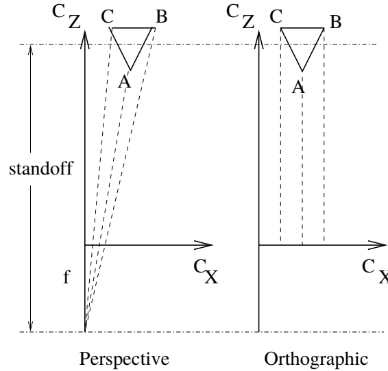
Figure 13.12: Perspective projection (left) versus orthographic (right).
