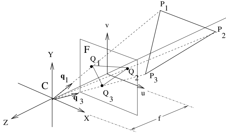
Figure 13.21: A simple case for pose estimation: a triangle P_1P_2P_3 with sides of known length in 3D is observed in the u v image plane as triangle Q_1Q_2Q_3 . The 3D positions of points P_j can be computed from the observed image points Q_j . The pose of an object containing the P_j can then be determined relative to the camera coordinate system. The focal length f is the distance from the center of projection to the image plane. Coordinates of the image points are Q_j = [u_j, v_j, -f] relative to the camera coordinate system \mathbf{C} .
