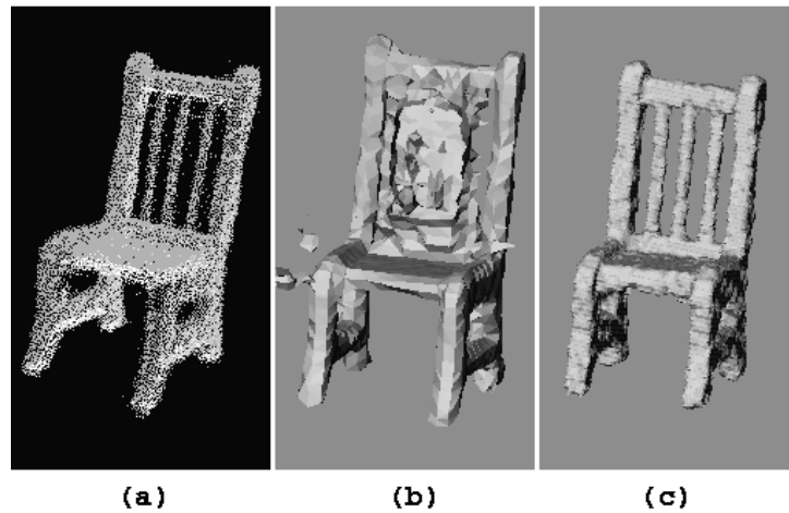
Figure 13.33: The registered range data for a chair object (left), problems that can occur in reconstruction (middle), and a topologically correct rough mesh model (right). Courtesy of Kari Pulli.
