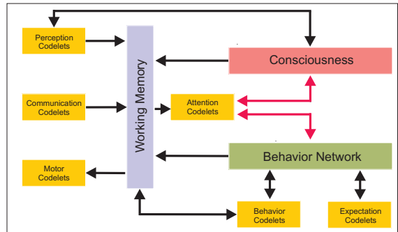
Figure 2: CAV’s Architecture
