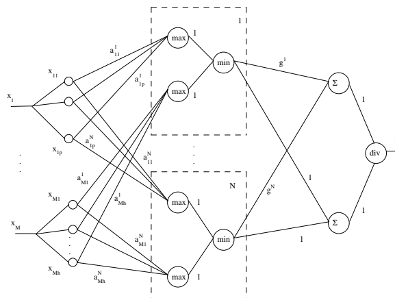
Figura 24: Controlador Neural Fuzzy
