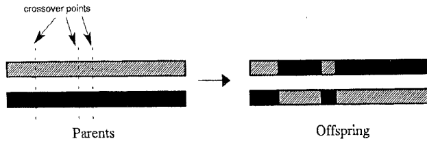
Fig. 7. Example of multipoint crossover, ( m = 3 )
