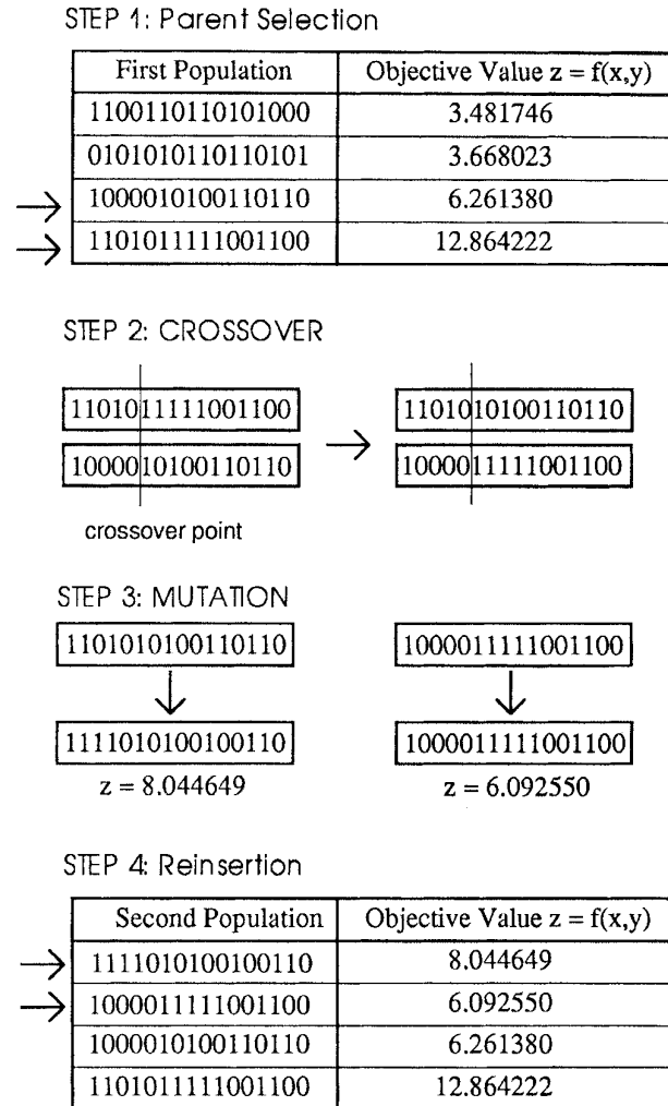
Fig. 5. Generation to generation.
