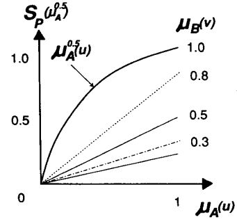
Fig. 4. Approximate reasoning: generalized modus ponens with Larsen's product operation rule.
