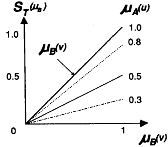
Fig. 9. Approximate reasoning: generalized modulus tollens with Larsen's product operation rule.
