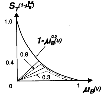
Fig. 8. Approximate reasoning: generalized modulus tollens with Larsen's product operation rule.
