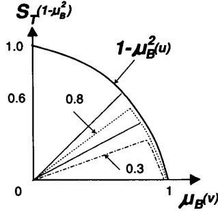
Fig. 7. Approximate reasoning: generalized modulus tollens with Larsen's product operation rule.
