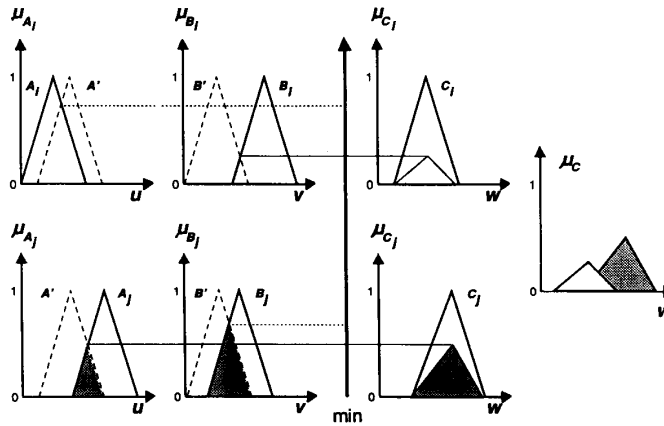
Fig. 11. Graphical interpretation of Lemma 2 under \alpha_i^{\wedge} and R_p .
