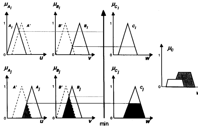
Fig. 10. Graphical interpretation of Lemma 2 under \alpha_i^{\wedge} and R_c .
