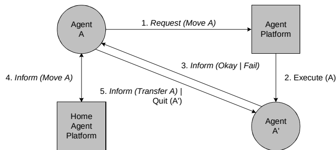
201 Figure 7: Full Agent Cloning Protocol
