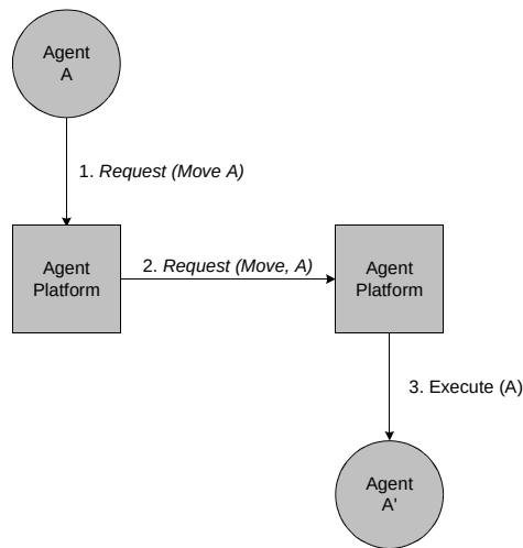
196 Figure 6: Simple Agent Cloning Protocol
