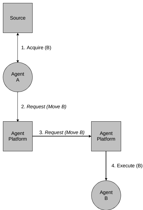
208 Figure 8: Simple Agent Invocation Protocol
