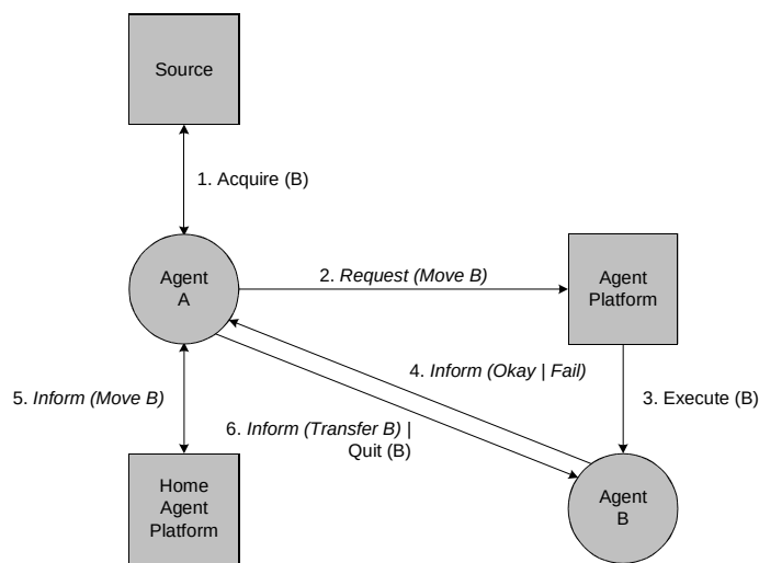
213 Figure 9: Full Agent Invocation Protocol
