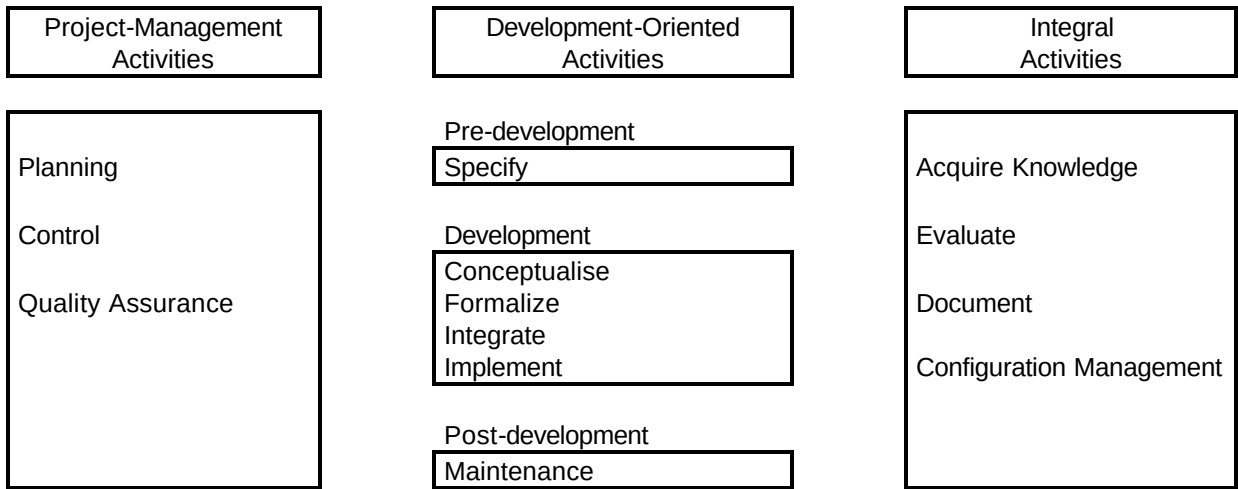
Figure 12: Ontology development process (proposition from [1])
