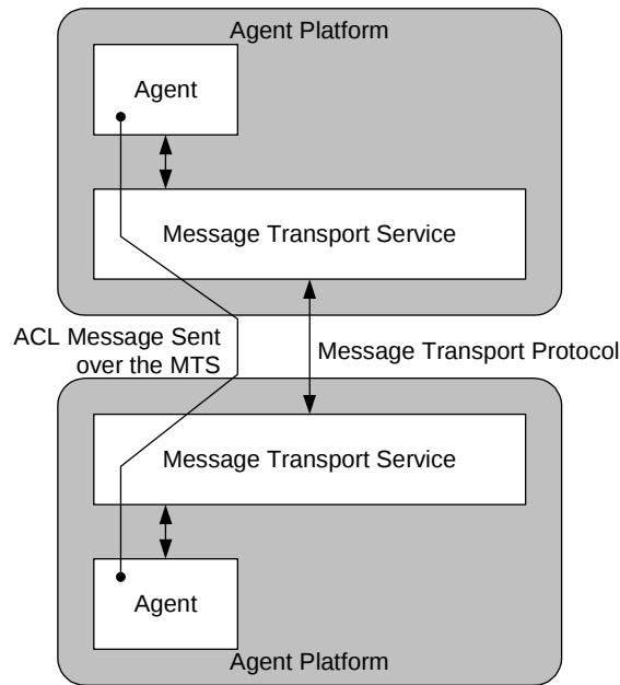
Figure 1: Message Transport Reference Model
