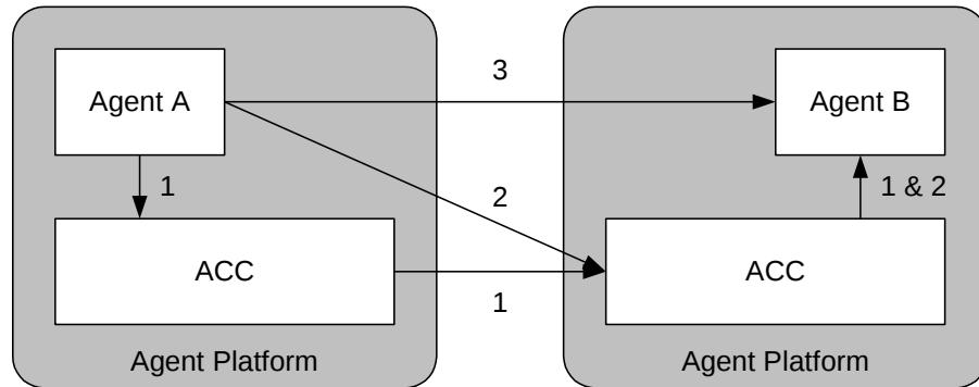
Figure 2: Three Methods of Communication between Agents on Different Agent Platforms 3
