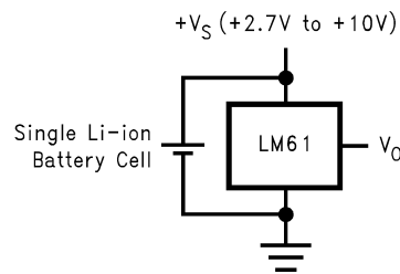
Figure 1. Full-Range Centigrade Temperature Sensor ( -30^\circ\text{C} to +100^\circ\text{C} ) Operating from a Single Li-Ion Battery Cell
