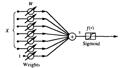
Fig. 1. Adaline with sigmoid.
